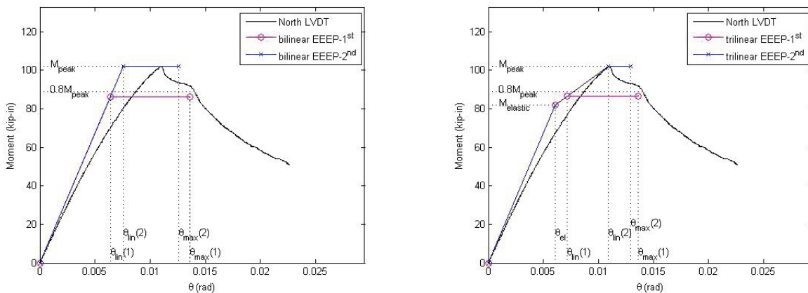
(a) bilinear EEEP models
